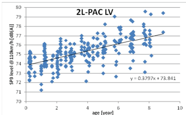
Figure 1. Example of a series of repeated SPB measurements (light vehicles) on 2L-PAC on several locations on Dutch highways. In total the data set covered nine years and are distributed over more locations.
